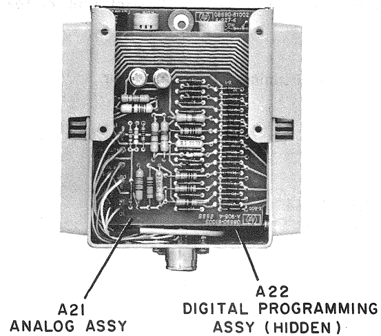
Figure 4. Digital Frequency Controller Interior View (Part of Change 1)
